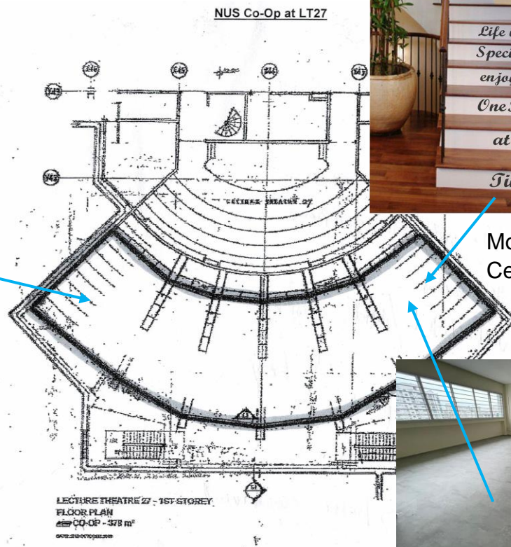
Selected areas with Vinyl Floor, Cement design
